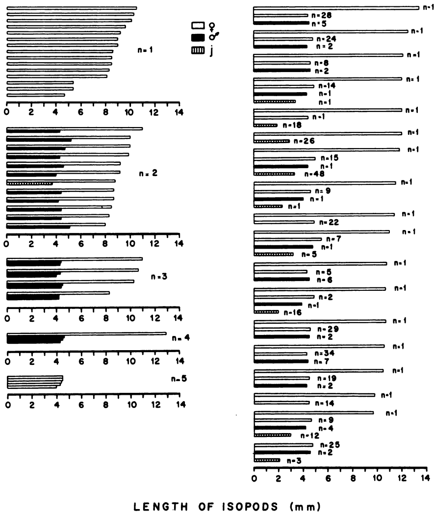
FIGURE 3. Number, size and sex of the isopods found in the mantle cavity of Mytilus chilensis in Gregorio Bay.
